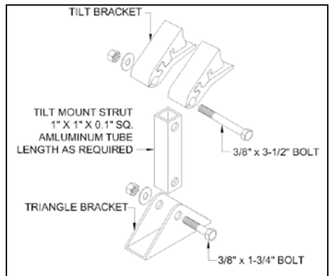
Rear hinge and strut Diagram 2
