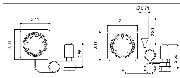
"Uni LH" Remote control depth 2 1/8"
