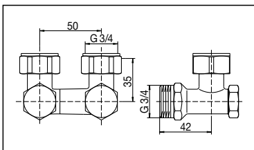
ZB angle pattern pre- set isolating fitting 3/4" (3/4" collar nut x 3/4" male thread) Item no. 101 62 12
