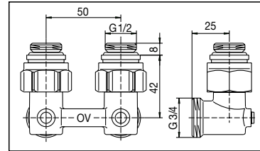
ZB angle pattern isolating fitting 1/2" (1/2" x 3/4" all male thread) Item no. 101 58 84
