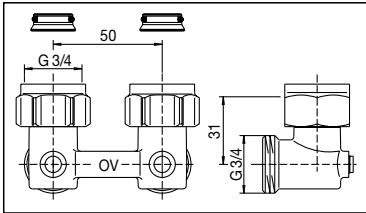
ZB angle pattern preset isolating fitting 3/4" (3/4" collar nut x 3/4" male thread) Item no. 101 58 14
