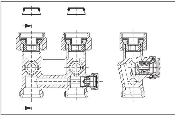
ZBU preset isolating fitting for two pipe systems for filling and draining, item no. 101 59 43
